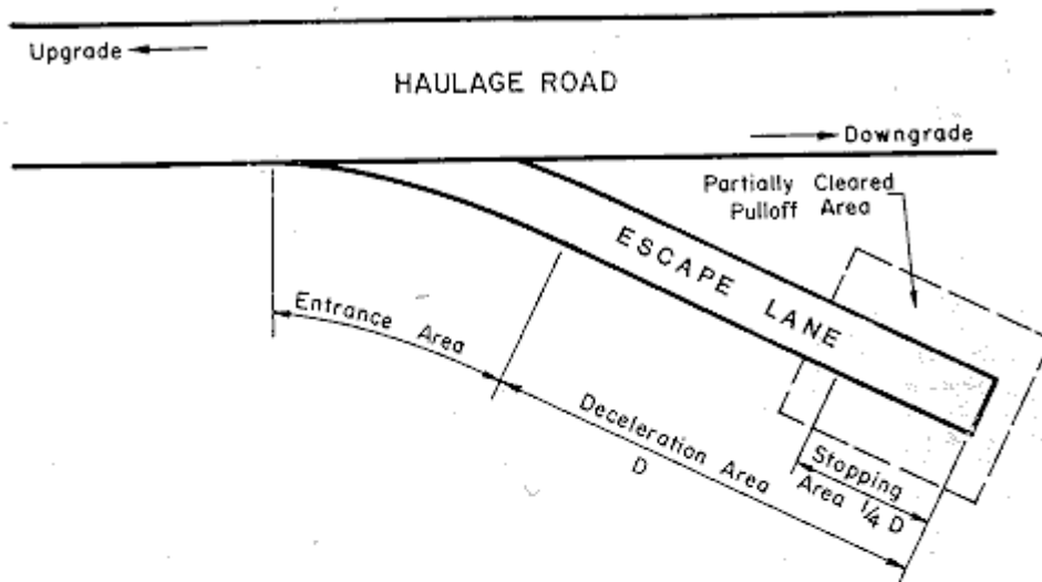
FIGURE 28. - Plan of haulage road escape lane.
